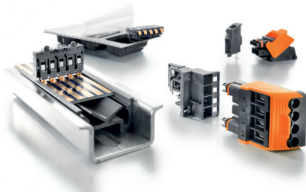
Integrated system bus in the TS35 standard top-hat rail
