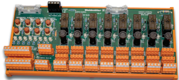
Pictured above is an 8 channel fused and jumper configurable I/O module with LED indication.
