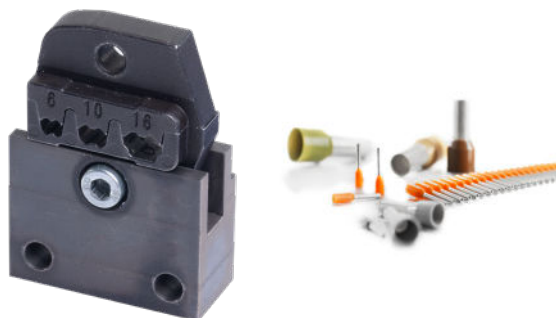
Crimping die set (ferrules) & base adapter Insert options are available for different conductor end finishes (e.g. PZ 16).
