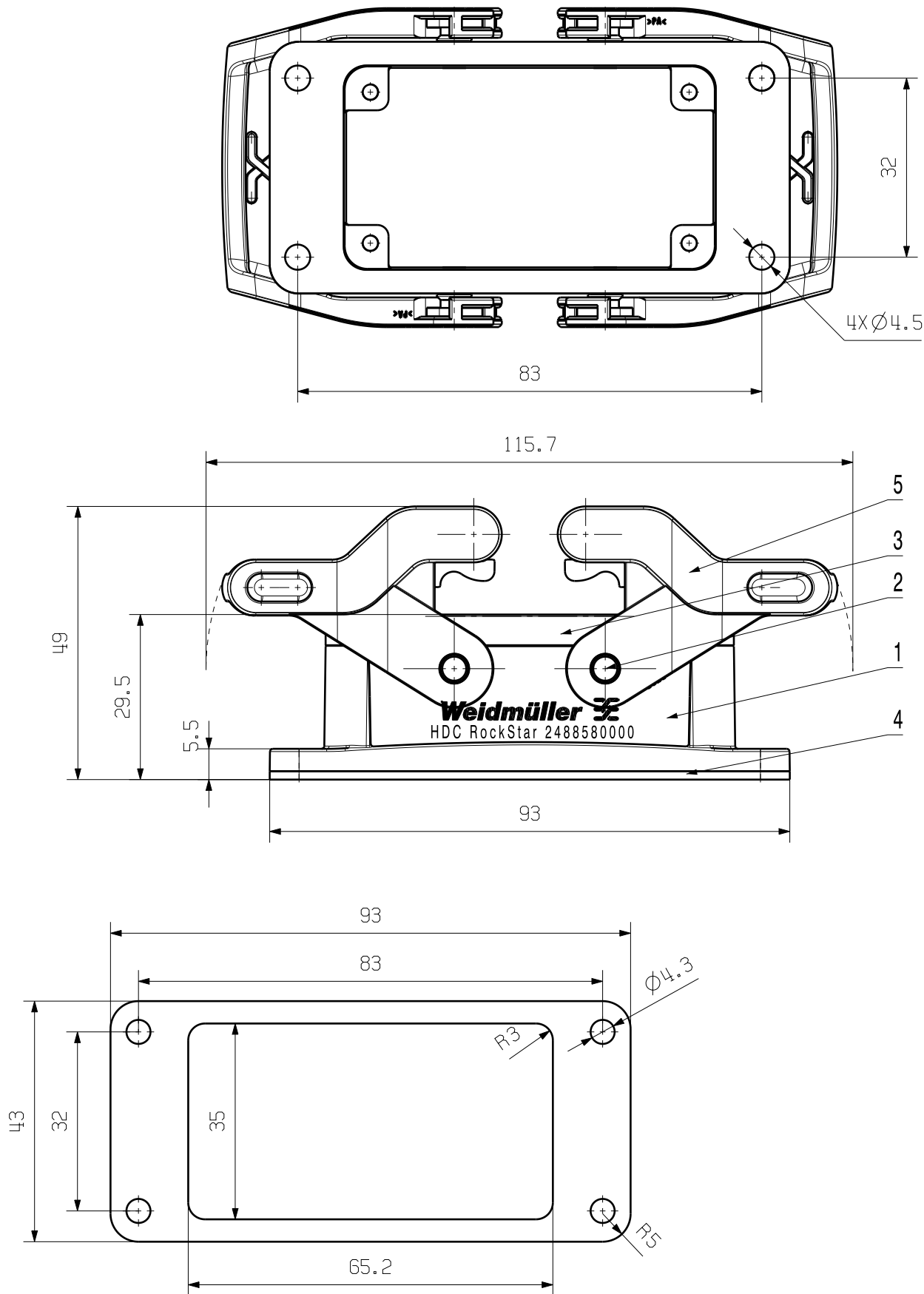
Mountageausschnitt Mounting cut-out
