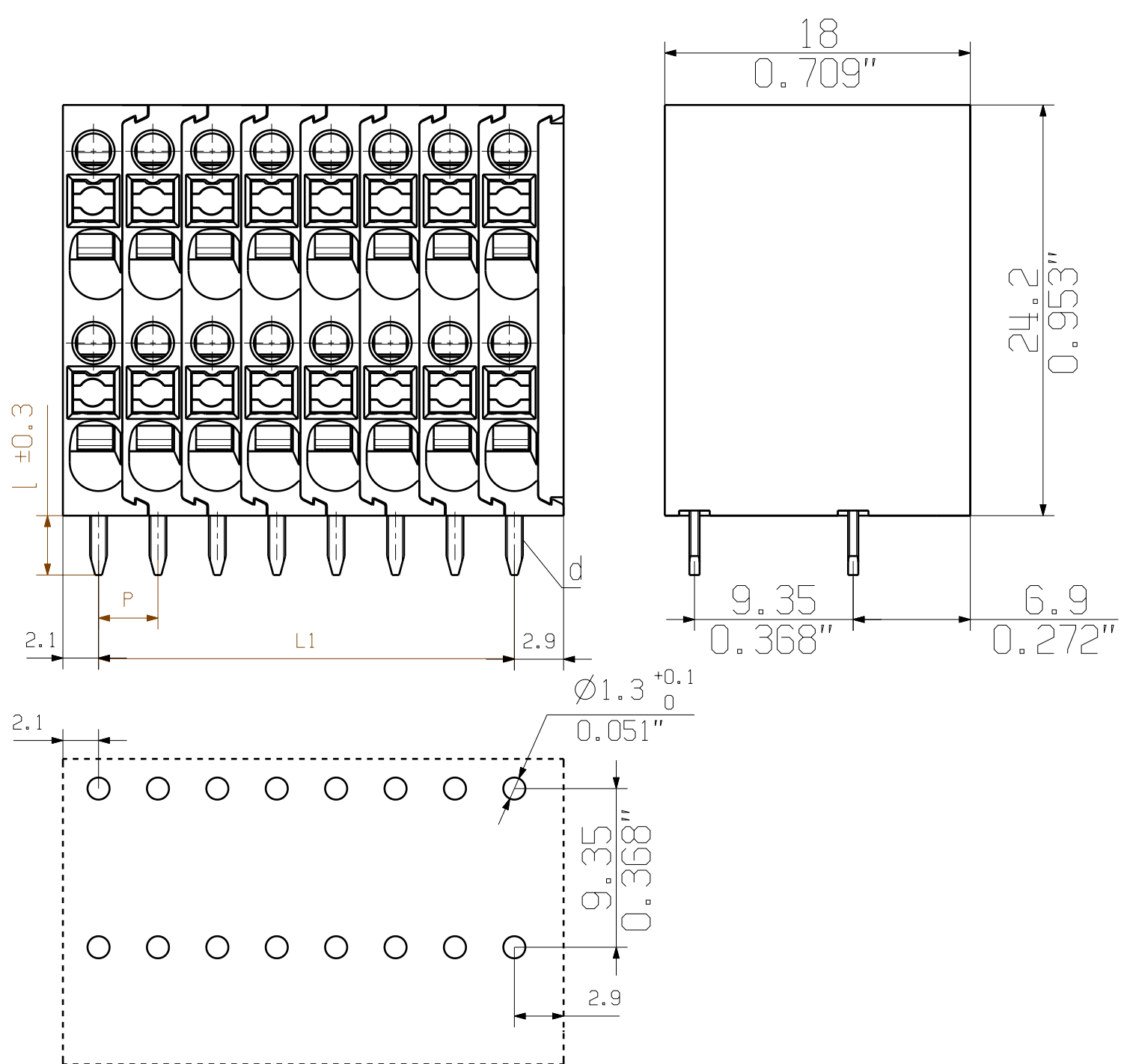
HOLE PATTERN
