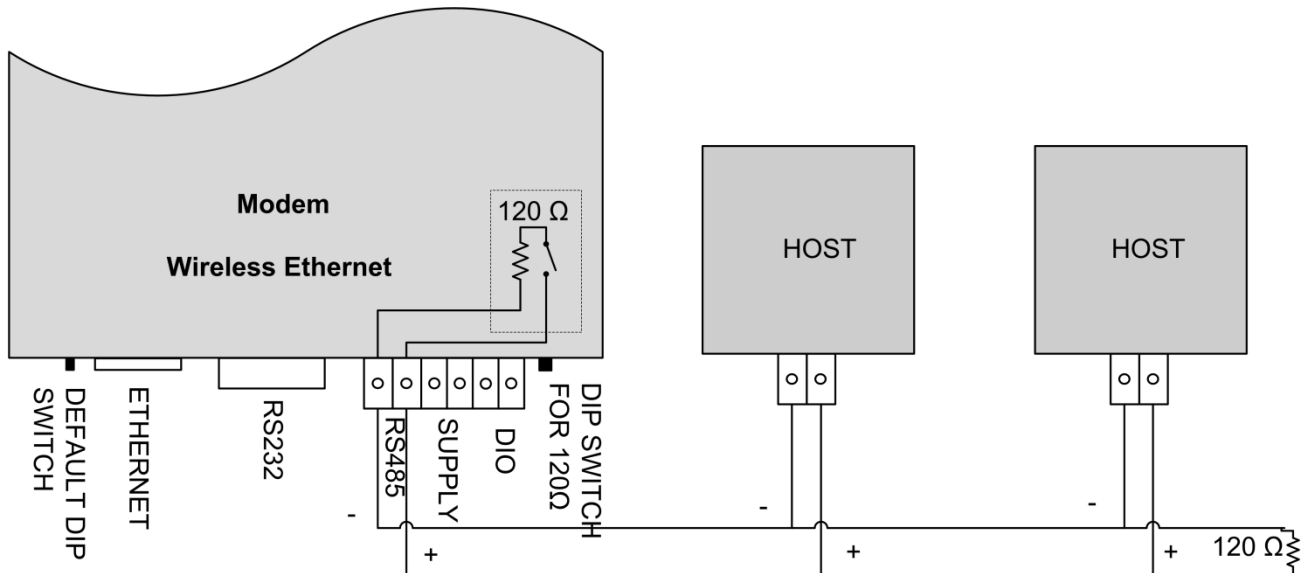
Figure 6 - Multidrop Serial
