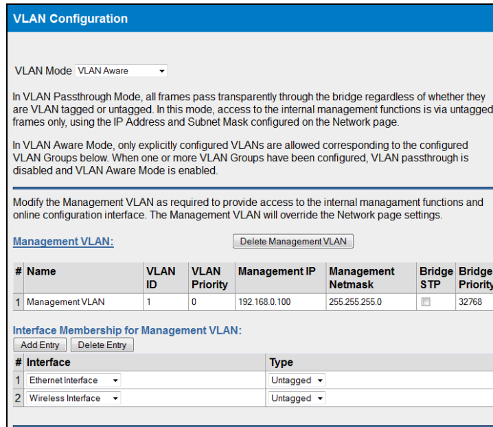
Figure 50 - VLAN Aware
