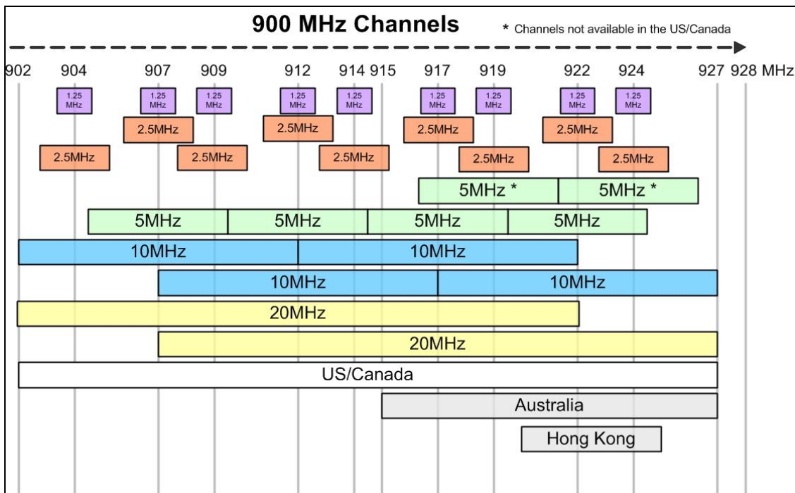
Figure 10 - 900MHz Channels
