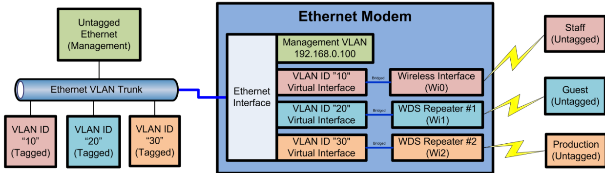
Figure 53 - VLAN Example 2
