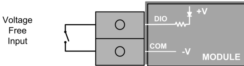
Figure 8 - DIO Input
