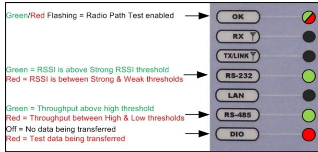
Figure 75 - Throughput Test LEDs
