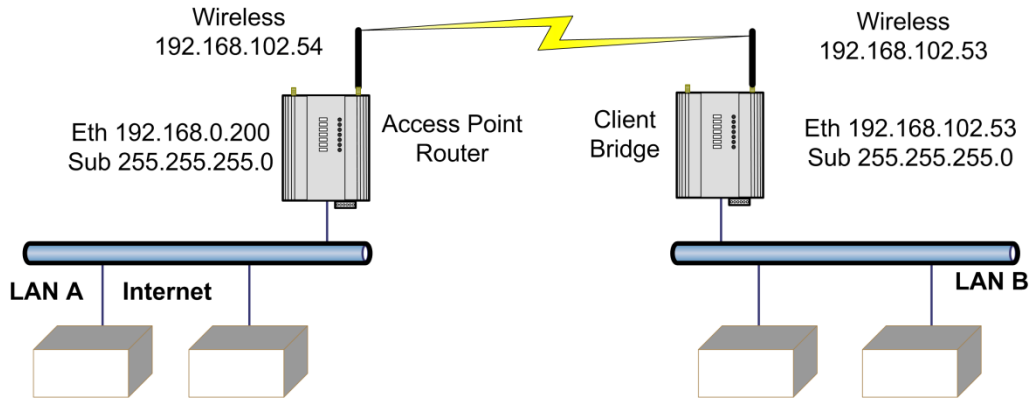
Figure 58 - Example Config 2
