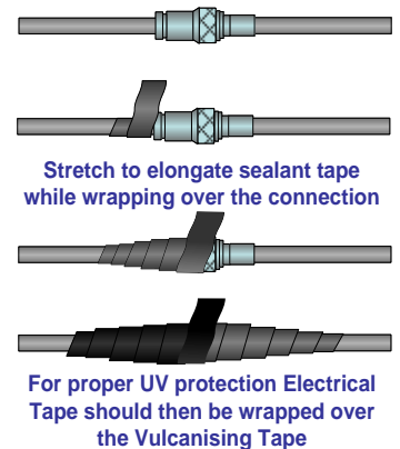
Figure 1 - Vulcanizing Tape
