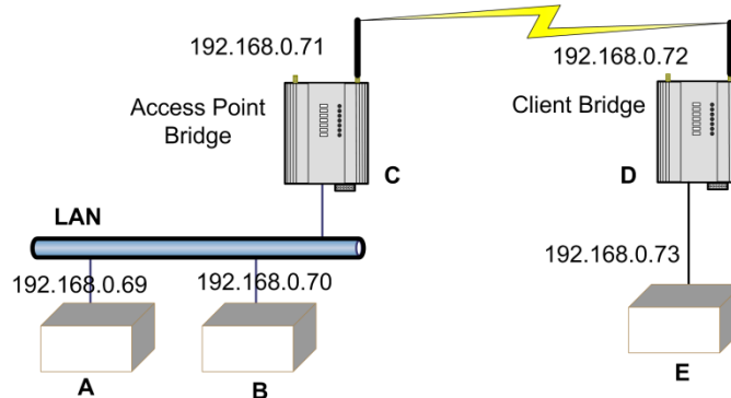
Figure 48 - Filtering Example
