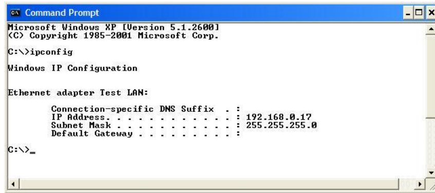
Figure 79 - Ipconfig
