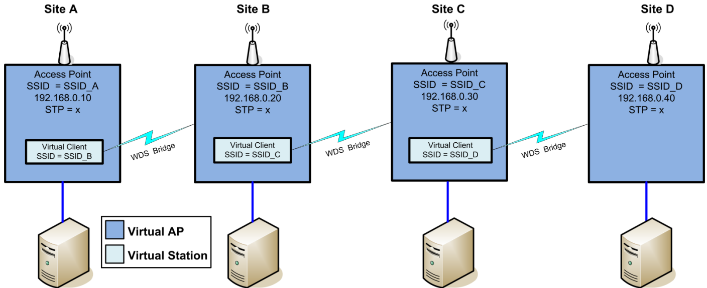
Figure 34 - Extending Range
