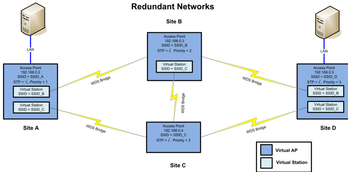
Figure 38 - WDS Redundancy
