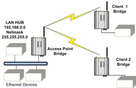
Figure 57 - Example Config 1
