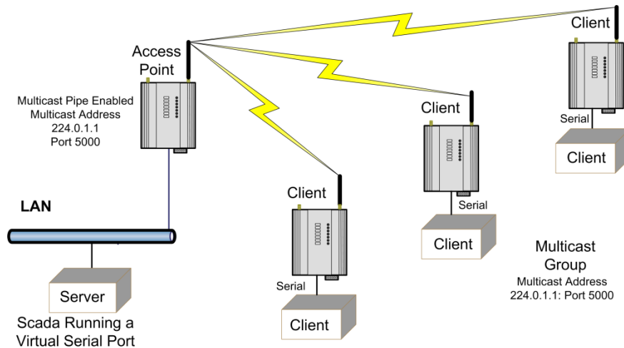
Figure 26 - Multicast Group
