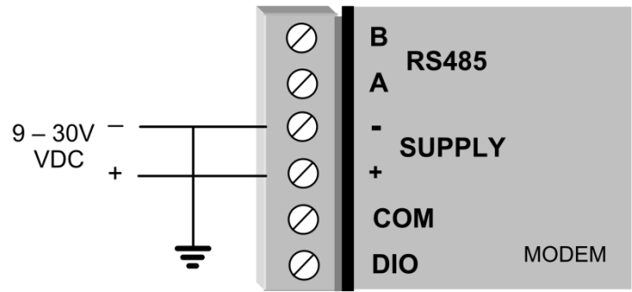
Figure 4 - Power Supply
