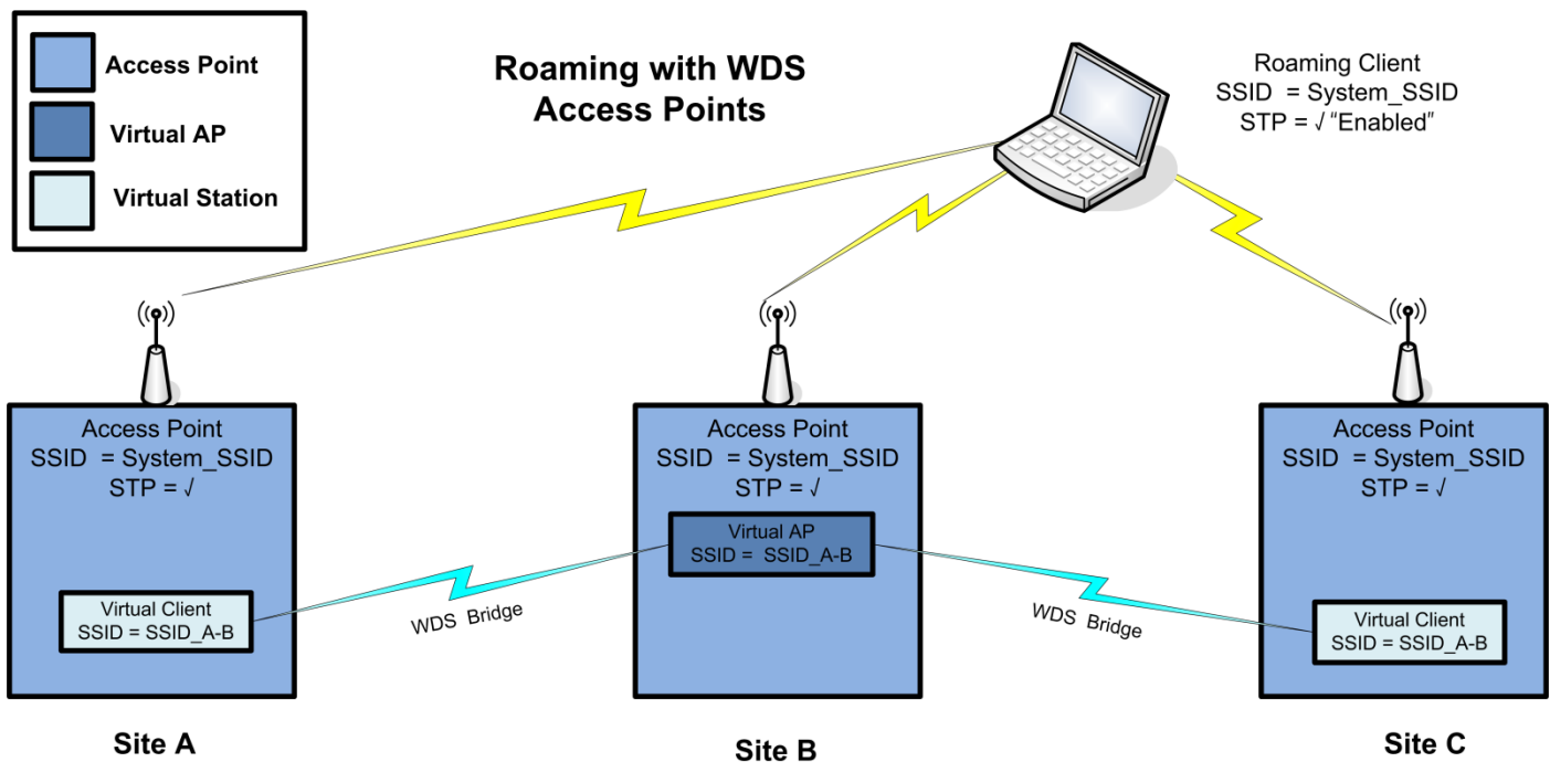
Figure 36 - WDS Roaming
