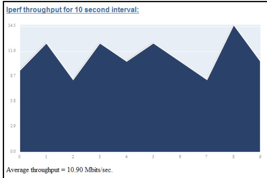
Figure 72 - Iperf Throughput
