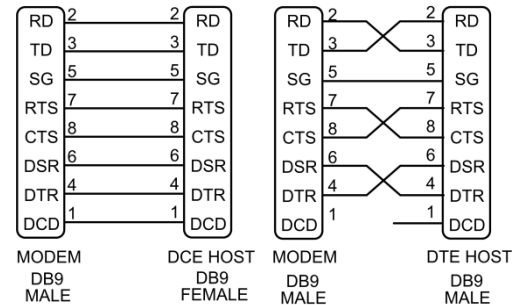
Figure 5 - Serial Cable
