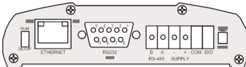
Figure 7 - End Plate
