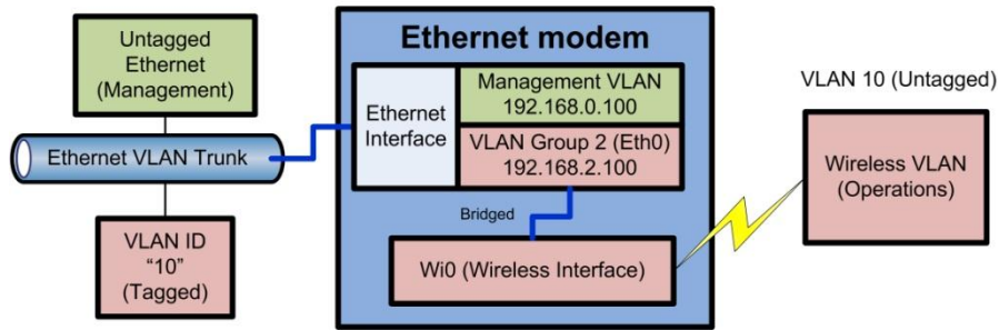
Figure 51 - VLAN Example 1
