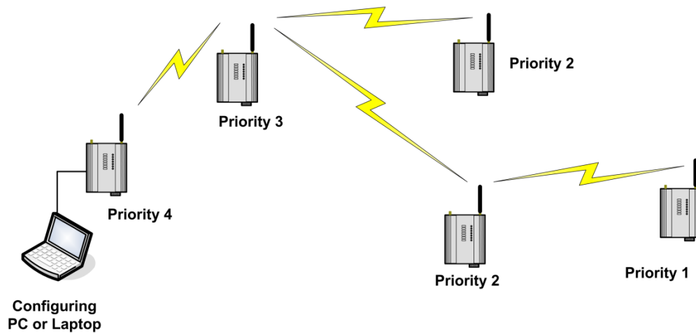
Figure 76 - Remote Configuration
