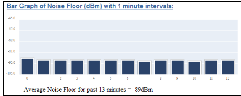
Figure 65 - RX Noise Floor Minutes
