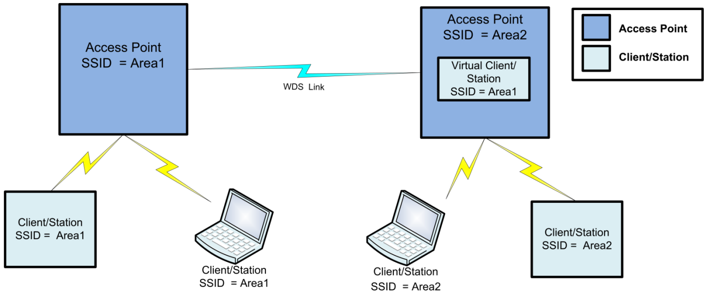
Figure 33 - WDS Repeaters
