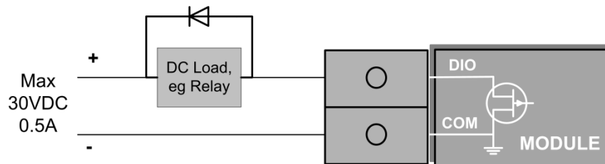
Figure 9 - DIO Output
