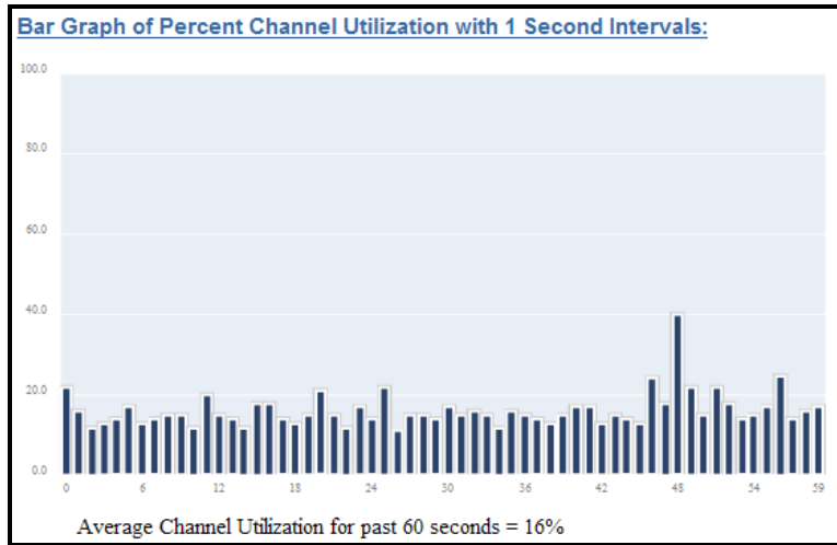
Figure 62 - Channel Utilization
