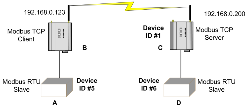
Figure 29 - Modbus
