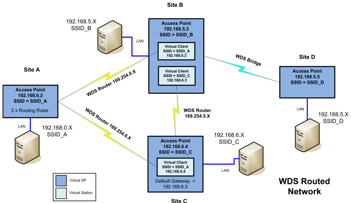
Figure 41 - WDS Routed
