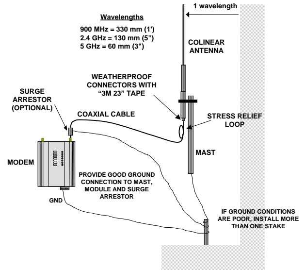
Figure 2 – Collinear Antenna
