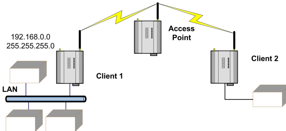
Figure 59 - Example Repeaters
