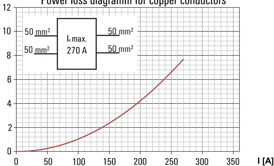
P [W] WPD 230 Power loss diagramm for copper conductors
