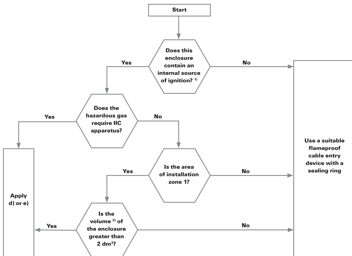
Fig 17: Selection chart for cable entry devices into flameproof enclosures for cables complying with item b)
