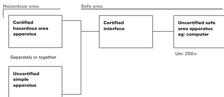
Fig 21: Individual systems
