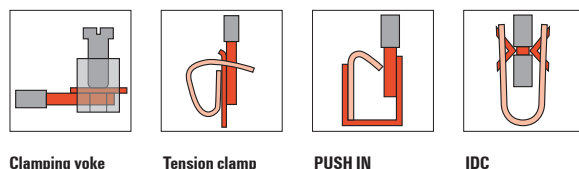
Fig 11: Connection technology
