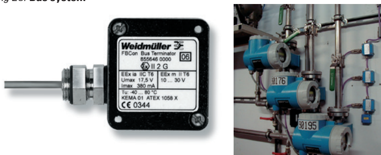
Fig 23: Bus system
