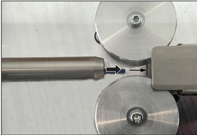
Figure 6.6 Inserting the wire correctly
