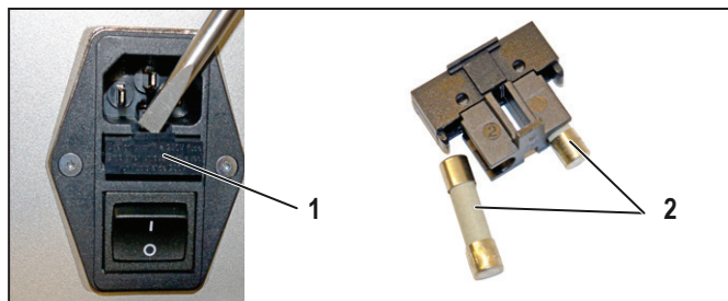
Figure 8.3 Fusibles
