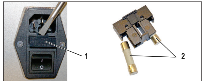
Figure 8.3 Fuses
