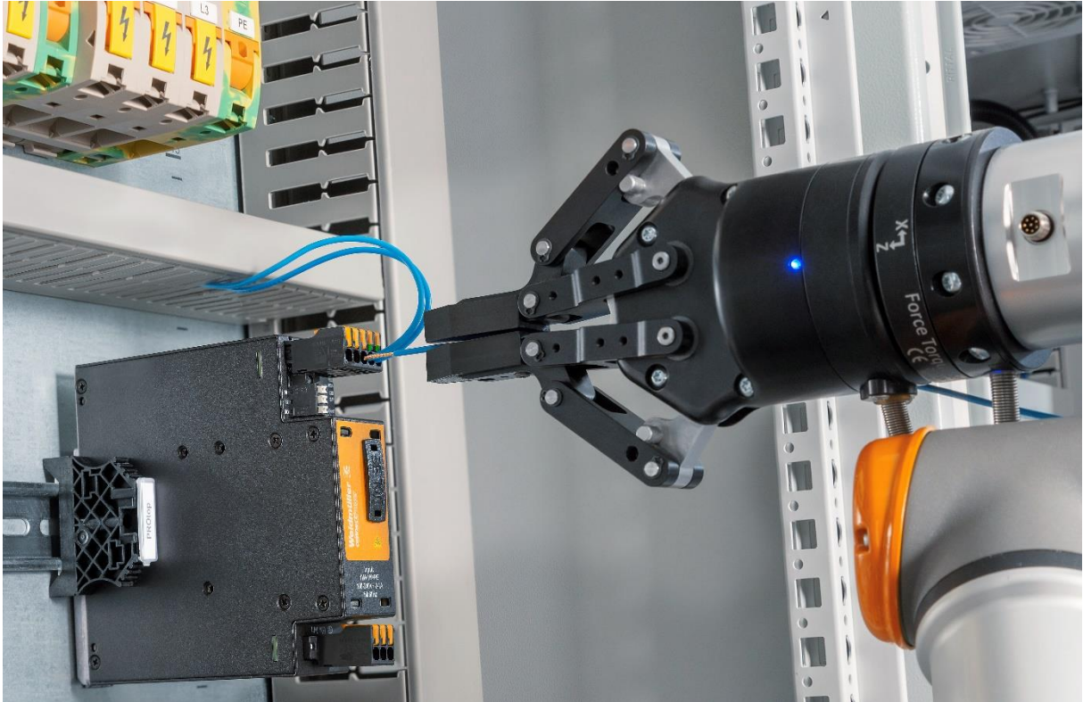
Image caption: OMNIMATE® 4.0 connectors are Ready to Robot
