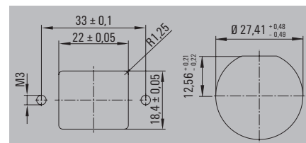
Normflansch
