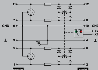
Complete module, direct earthing, with remote alert
