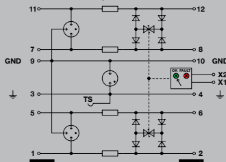
Complete module, indirect earthing, with remote alert
