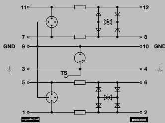
Complete module, indirect earthing
