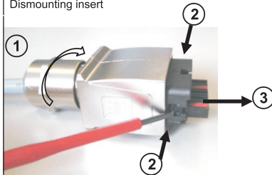
Dismounting insert
