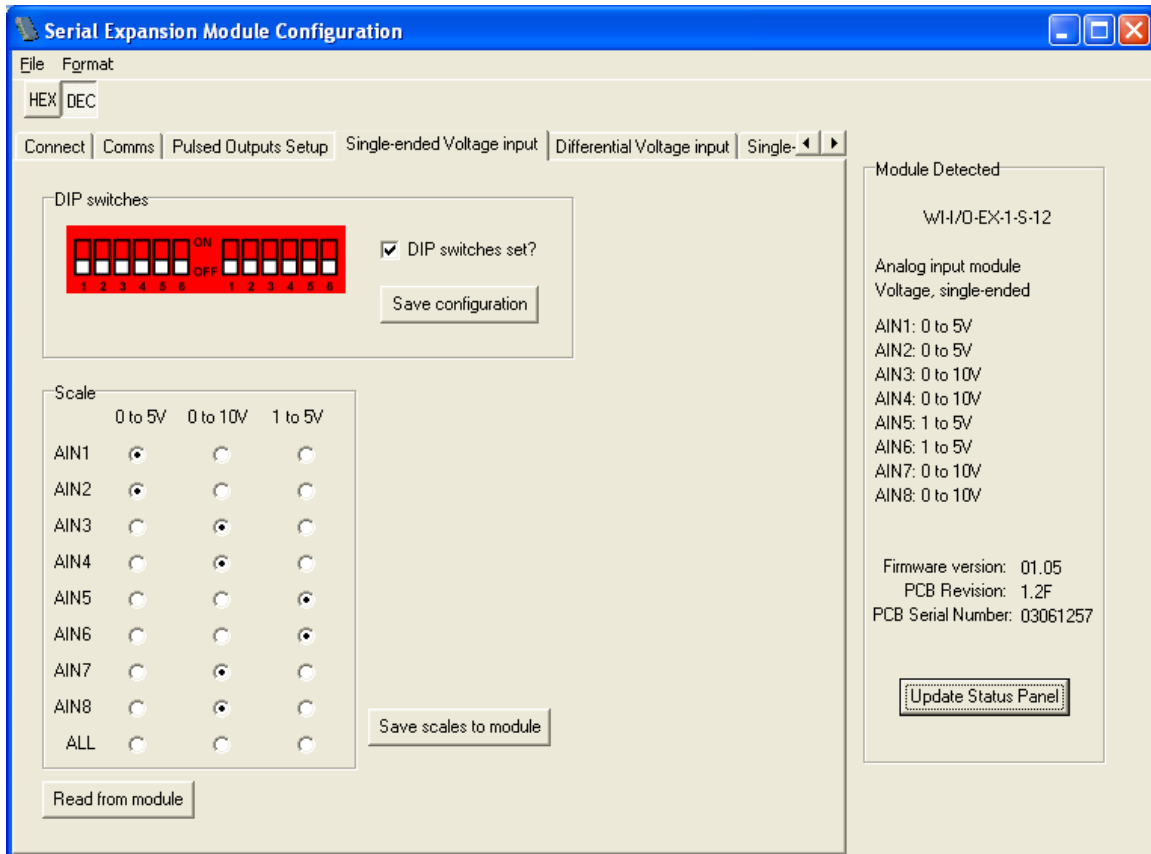
Figure 4-5: Setup page for single-ended voltage input.
