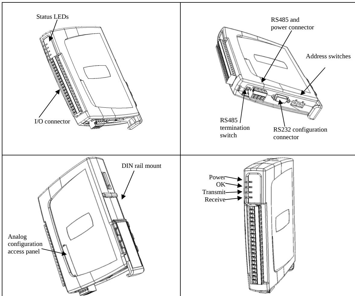
Figure 1-1: WI-I/O-EX unit with significant parts labeled.
