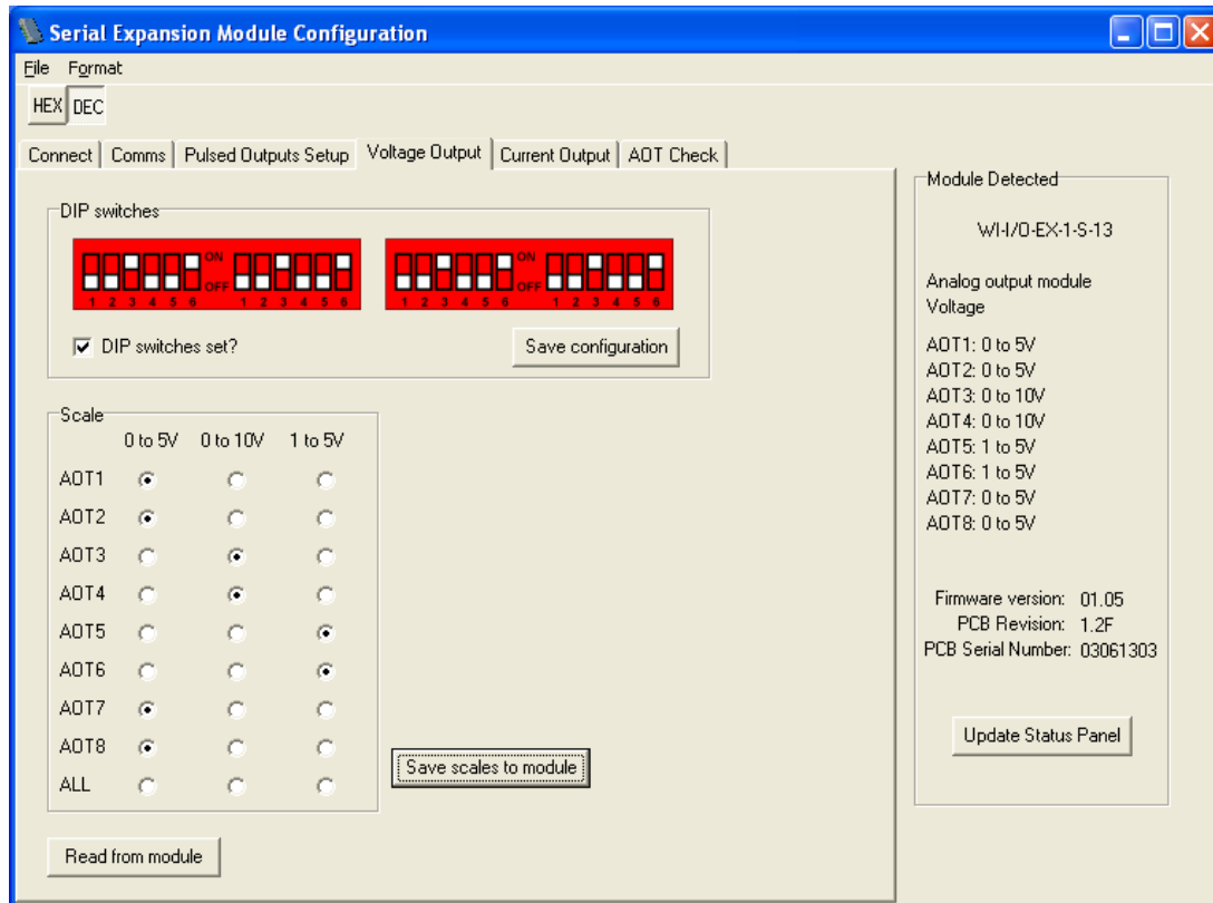
Figure 4-9: Voltage output setup page.
