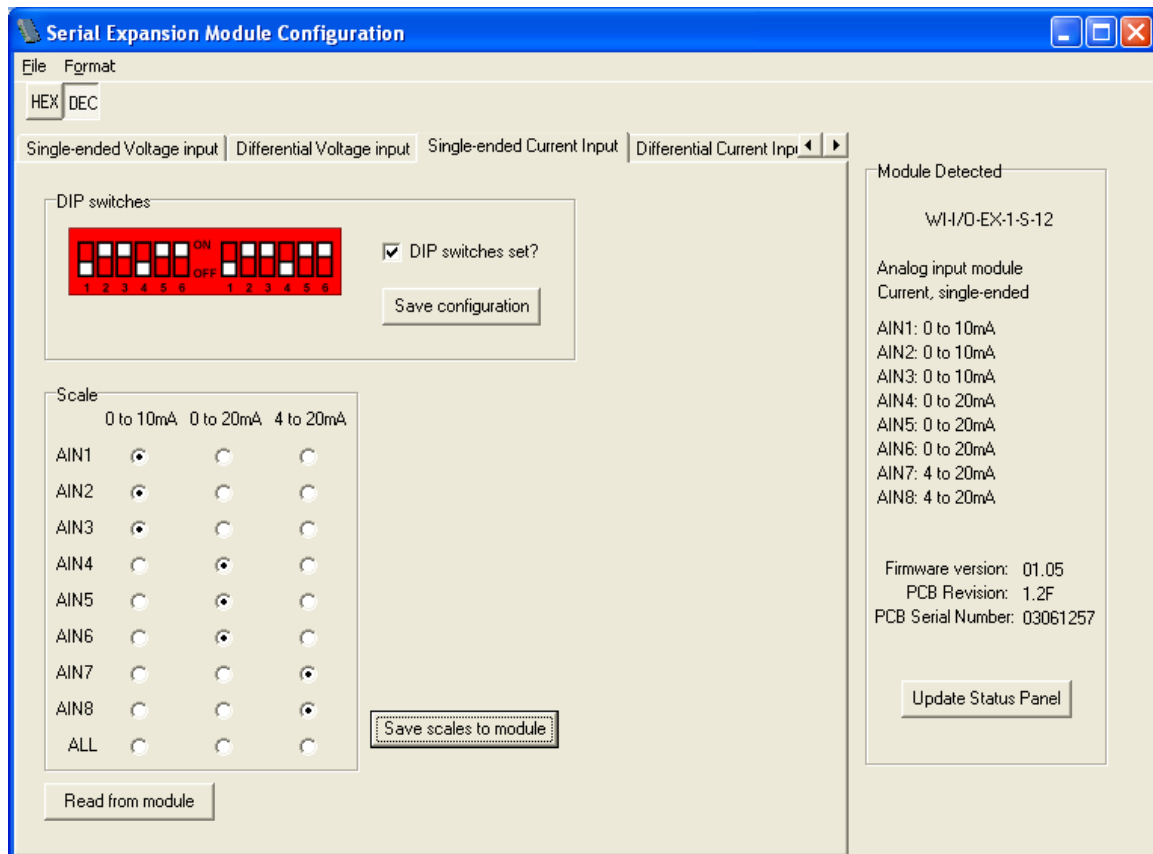
Figure 4-7: Setup page for single-ended current input.
