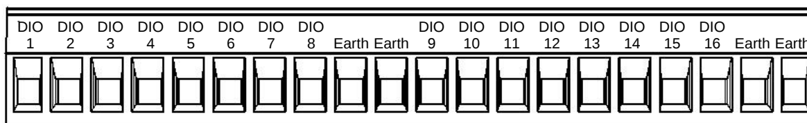
Figure 5-1: I/O terminal block for WI-I/O-EX-1-S-11.
