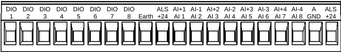
Figure 5-3: I/O terminal block for WI-I/O-EX-1-S-12.
