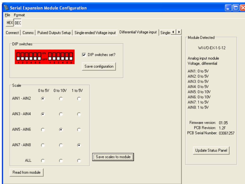
Figure 4-6: Setup page for differential voltage input.
