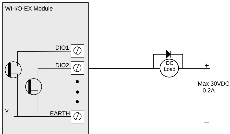
Figure 2-6: Connection of digital outputs.
