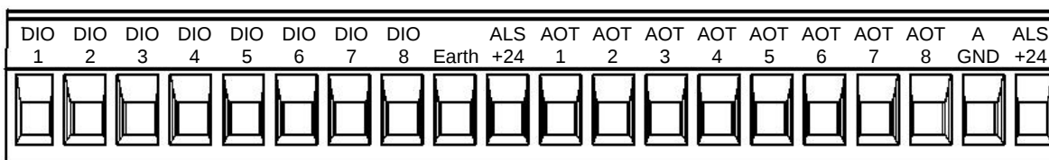
Figure 5-5: I/O terminal block for WI-I/O-EX-1-S-13.
