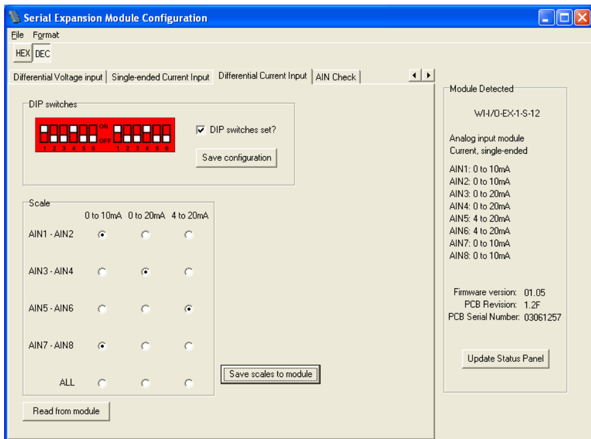
Figure 4-8: Setup page for differential current configuration.
