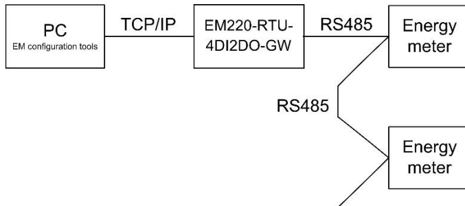
Fig: TCP/IP connection by gateway
