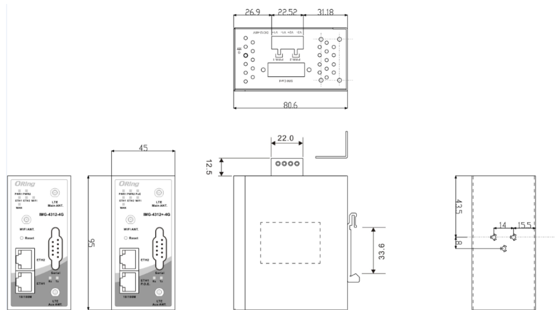
DIN-rail Kit Measurement (Unit = mm)
