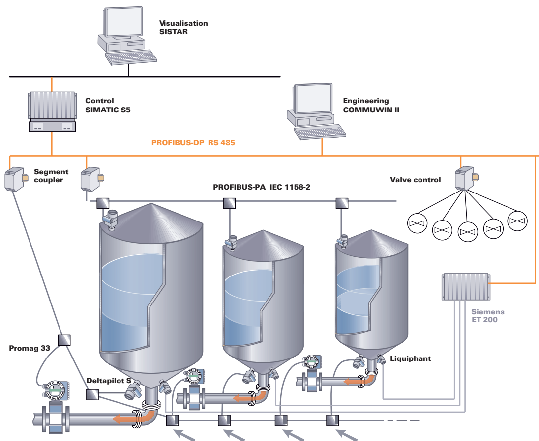
Fig 22: Fieldbus
