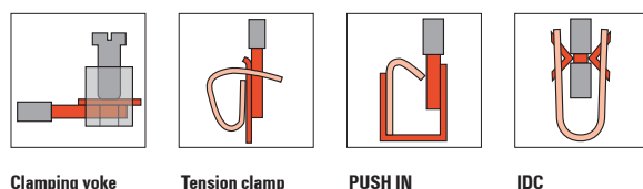
Fig 11: Connection technology
