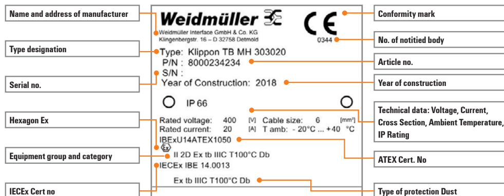
Fig 26: Example of the marking for a junction box
