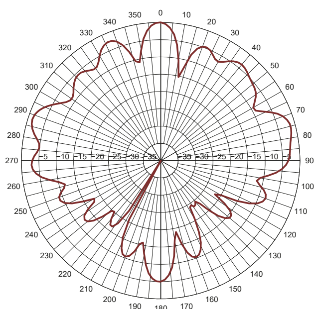
Elevation 5800 MHz
