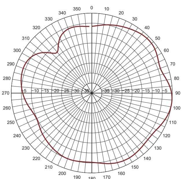
Azimuth 5800 MHz
