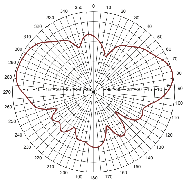
Elevation 2300 MHz
