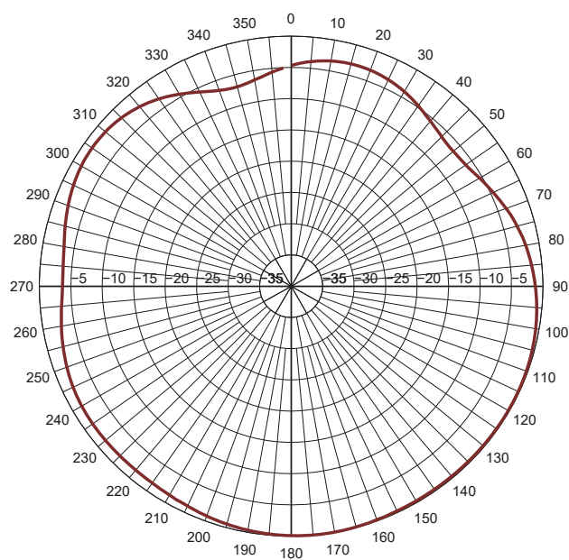
Azimuth 2300 MHz
