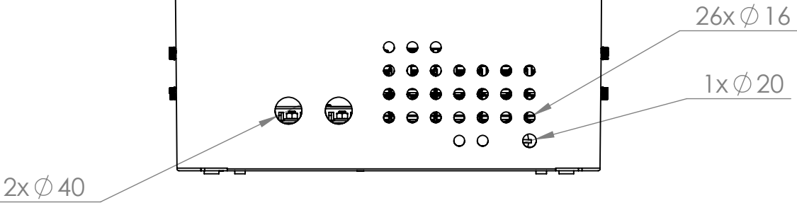
FRONT SIDE
