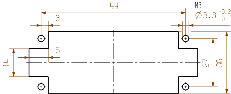
MOTAGEAUSSCHNITT MOUNTING CUT-OUT
