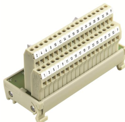
Example of Family RS F (w/ LPK connector)
