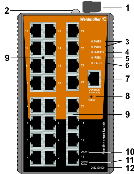
IE-SW-AL24M-24TX Front Panel View
