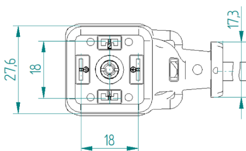
Dimensions Old
