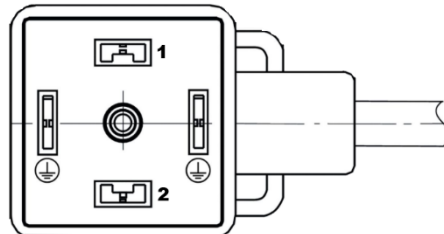
Pin assignment new
