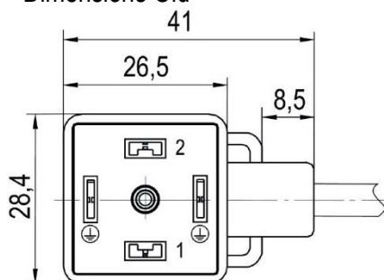
Dimensions Old
